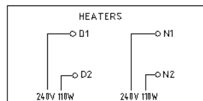
Connection diagram
