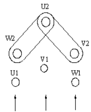
Connection diagrams Y Conn.
