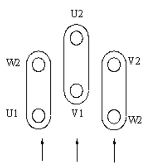
Connection diagram \Delta Conn.
